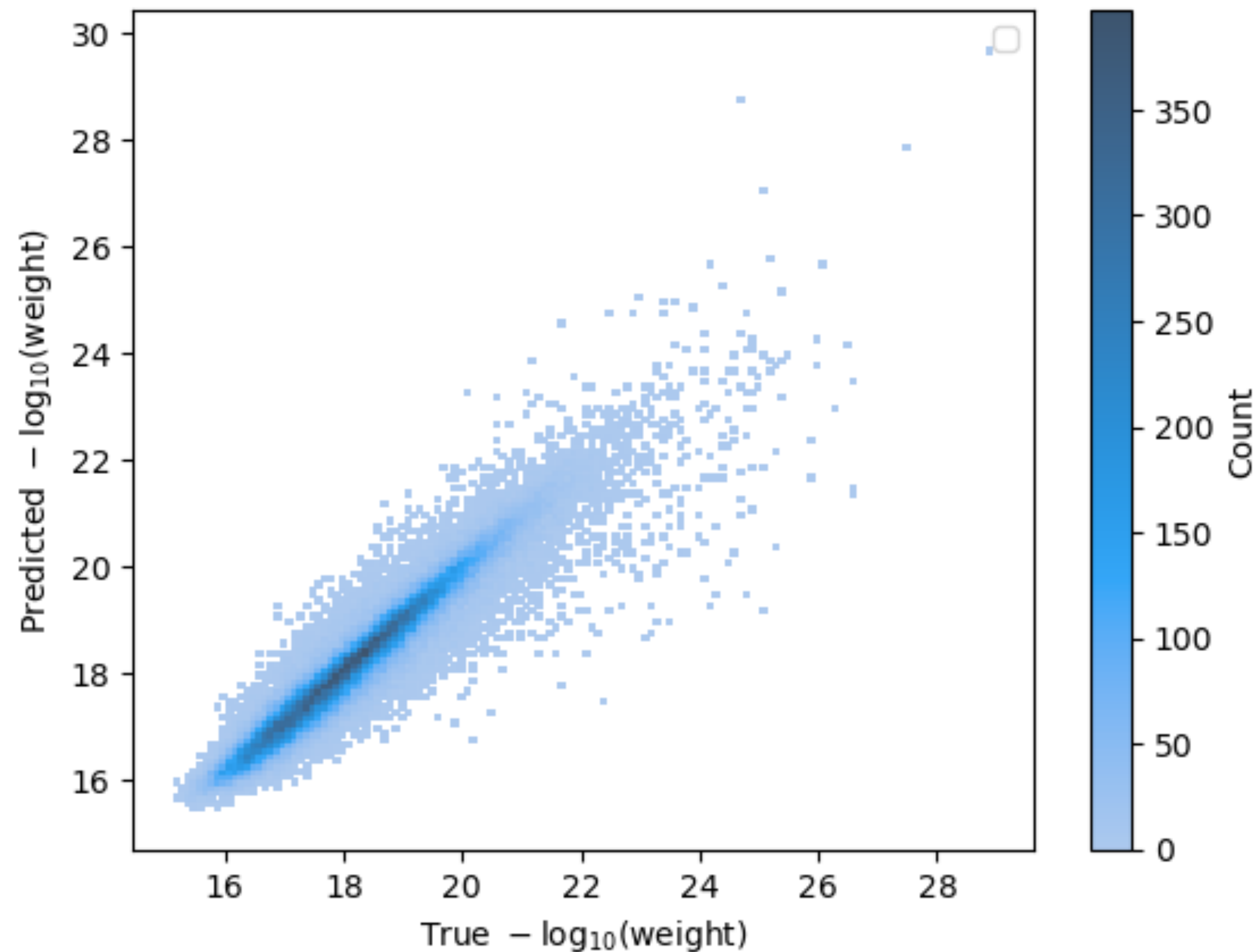
Feed-forward, true weights compared to predicted weights
