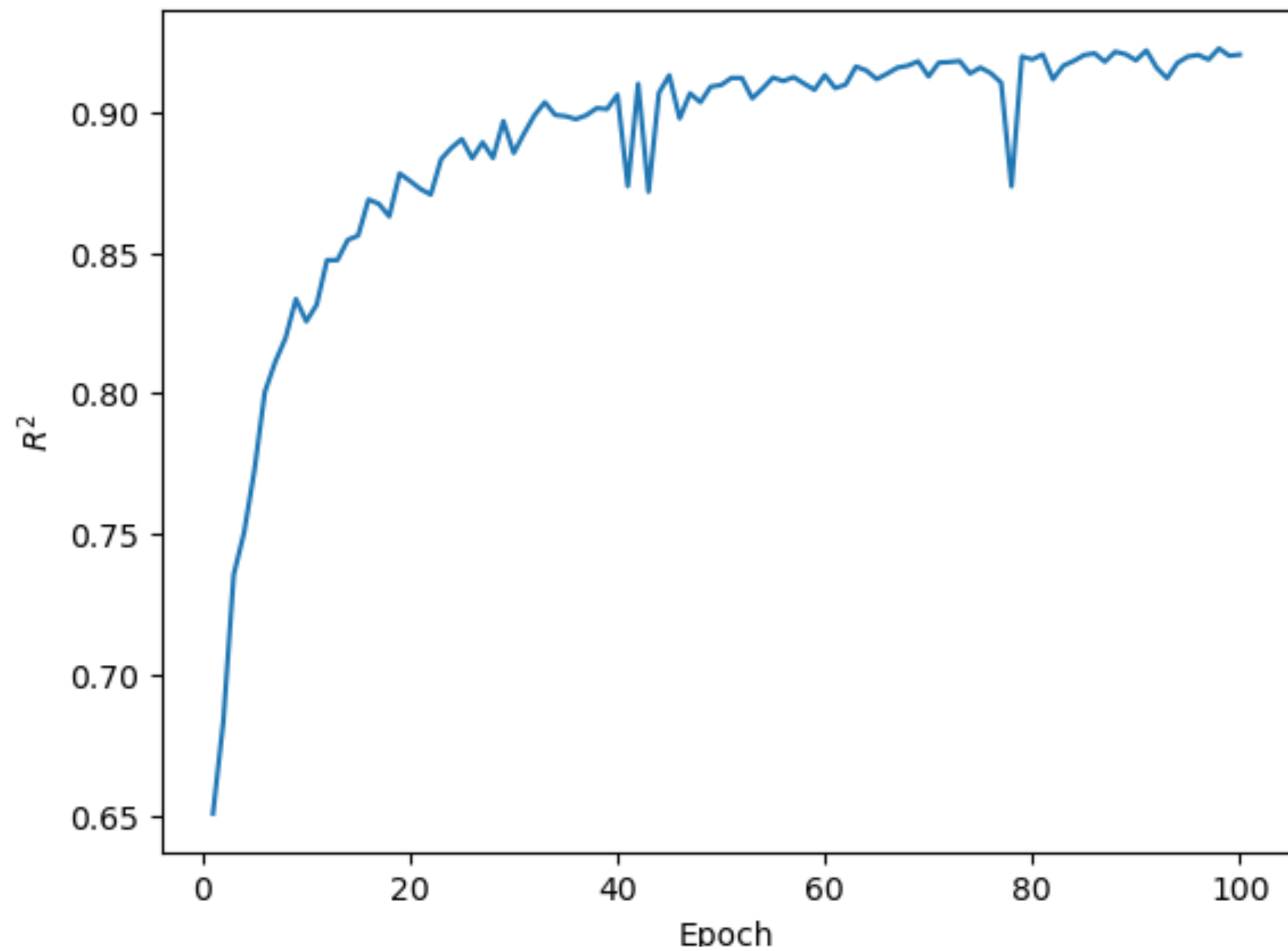
R^2 on validation data, FF network
