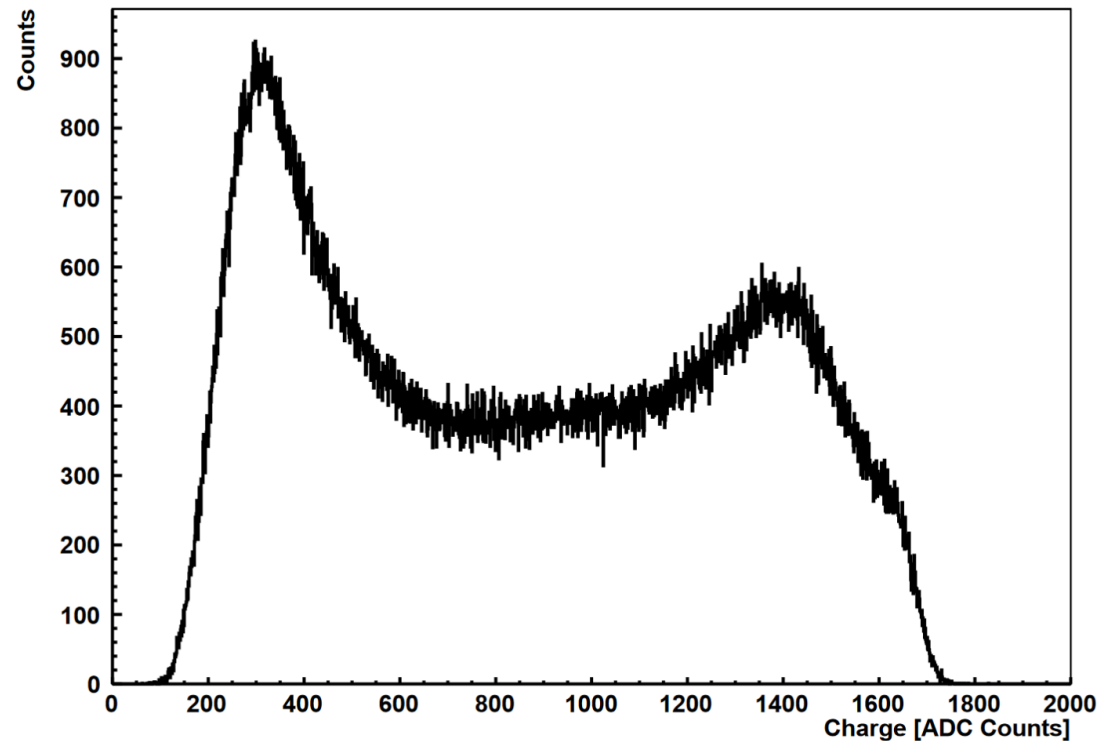
Strip Charge at 300V
