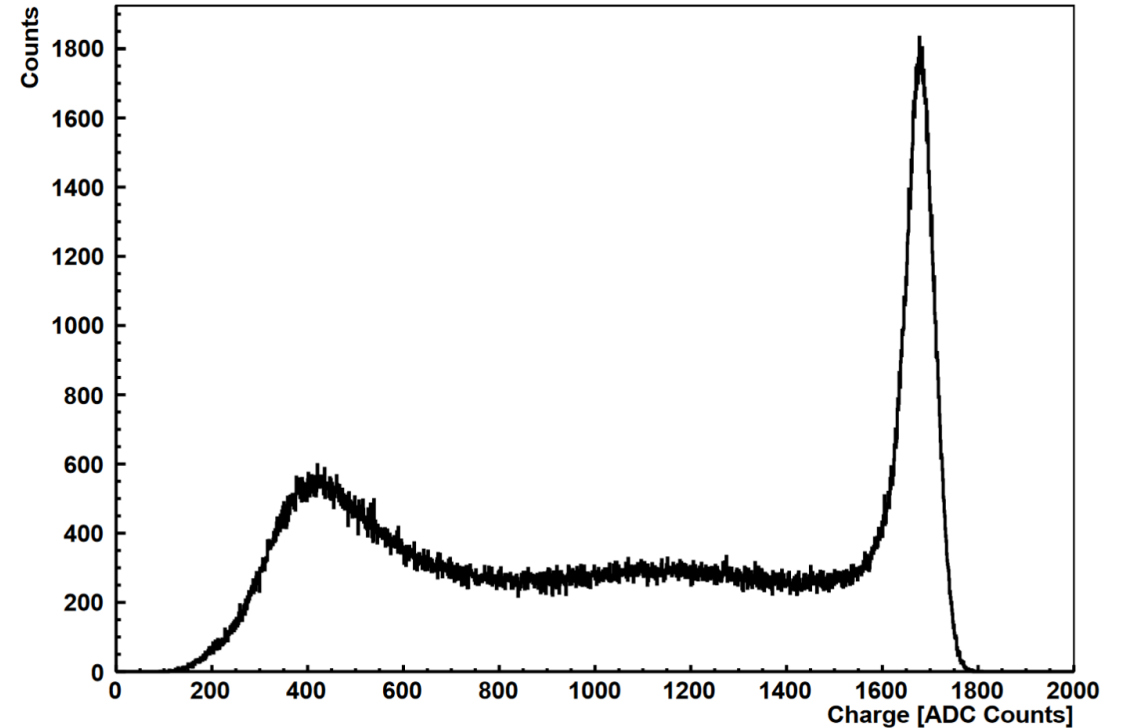
Strip Charge at 305V → Oversaturated
