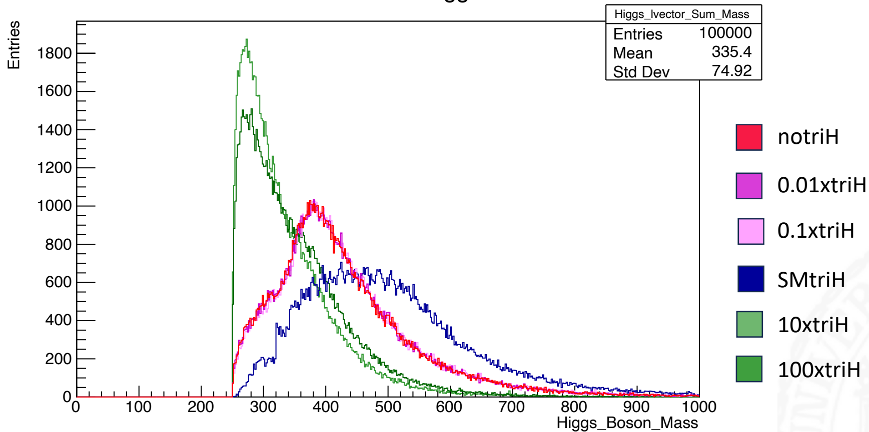
Mass of the Sum of the two Higgs Lorentz vectors
