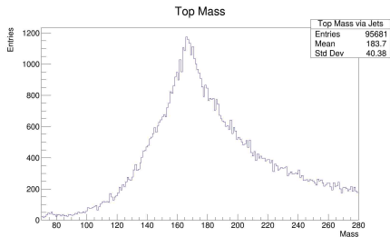
Top Mass via Jet Reconstruction
