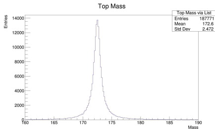
Top Mass via Particle List
