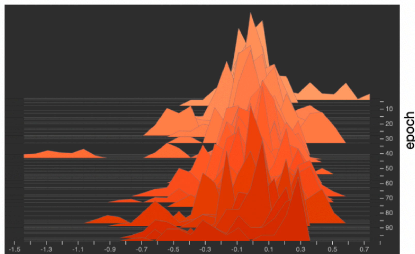
weight gradient
