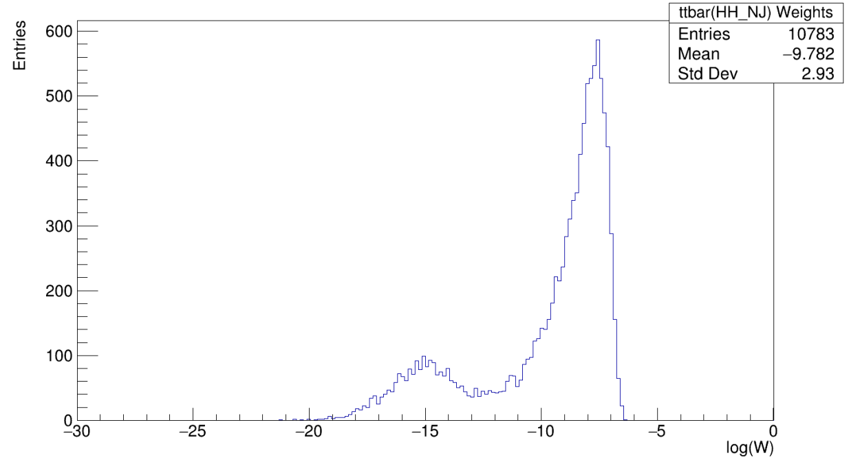
ttbar(HH_NJ) Weights
