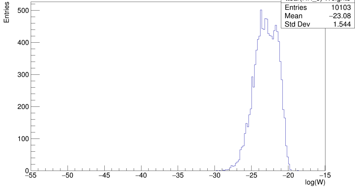
ttbar(HH_J) Weights
