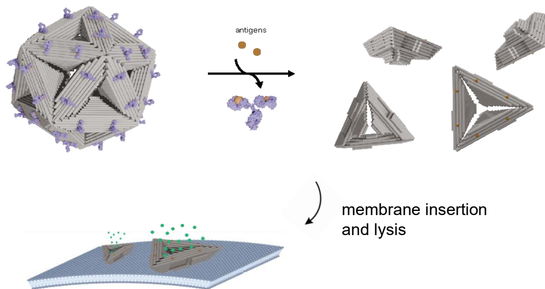
Figure 1: IgG-mediated stabilization and antigen-triggered disassembly of icosahedral DNA origami shells. The individual triangular building blocks, equipped with a potential pore-forming moiety, are designed to insert into the lipid membrane and cause lysis.
